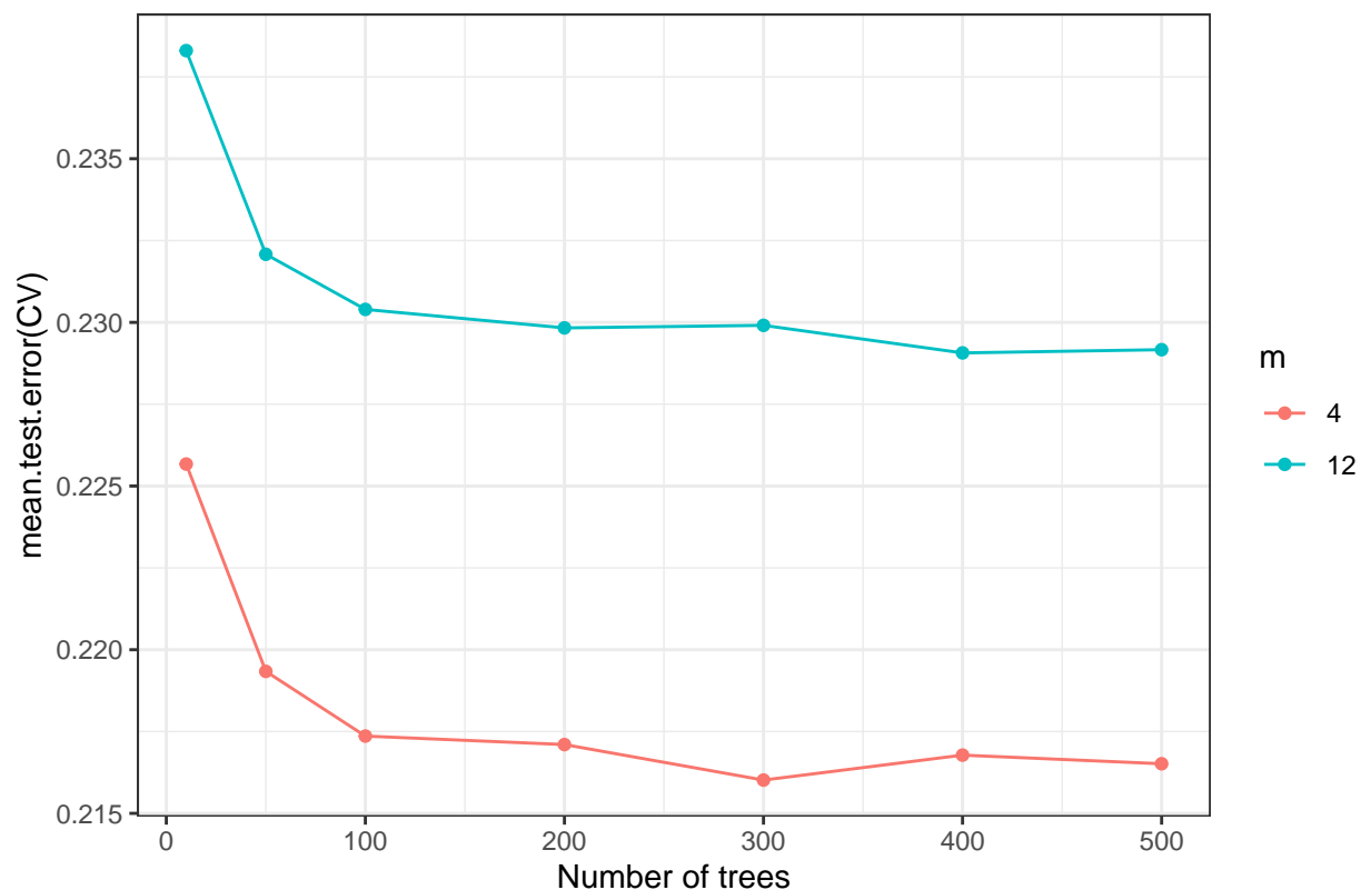
Mean test error from cross-validation
