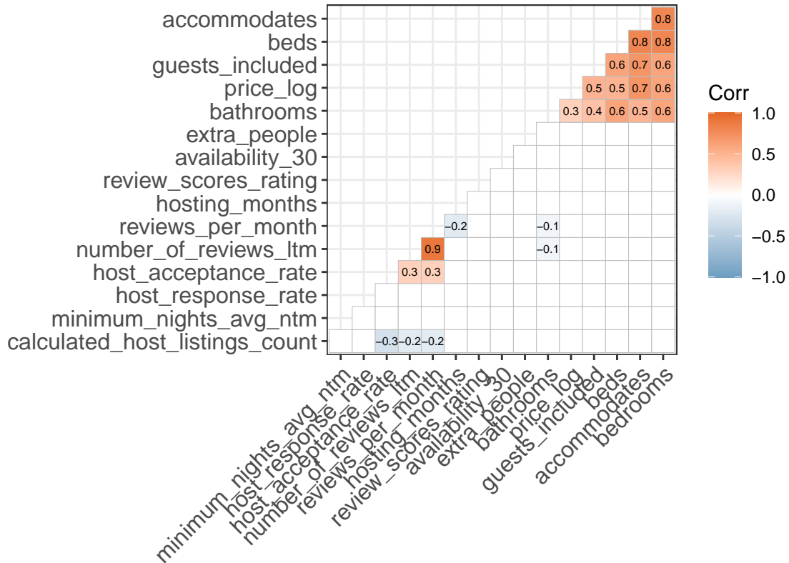
Correlogram of continuous variables
